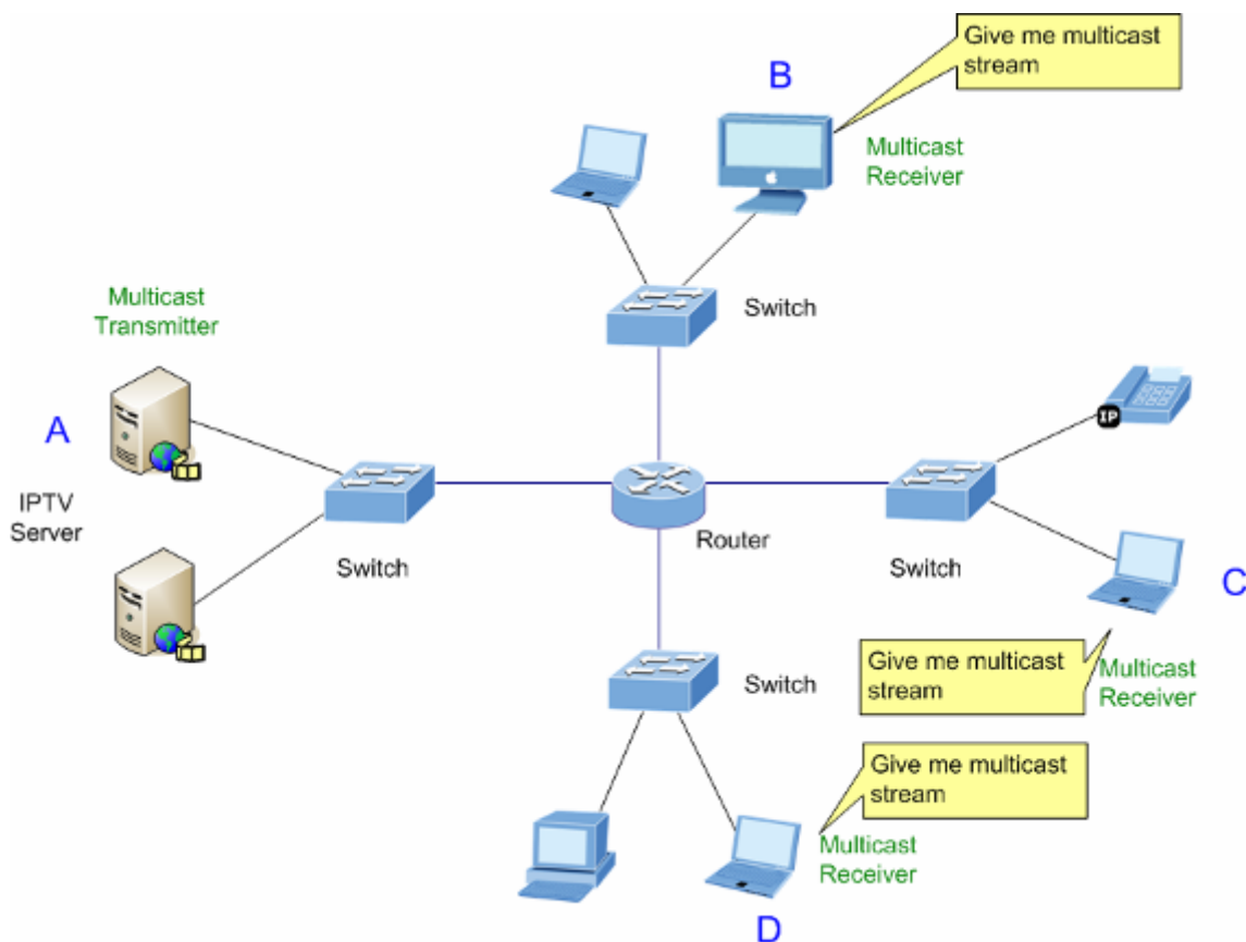
Figure 4-3-5-1: Multicast Service
