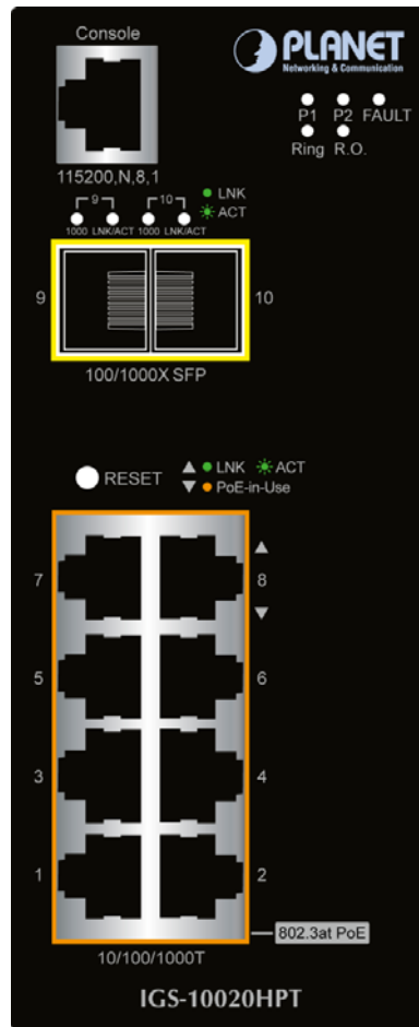
Figure 2-2: IGS-10020HPT Switch Front Panel
