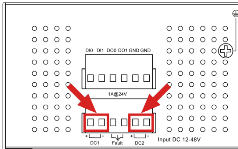
Figure 2-12: IGS-10020HPT Upper Panel
