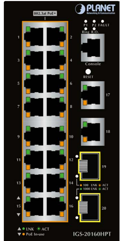
Figure 2-3: IGS-20160HPT Switch Front Panel
