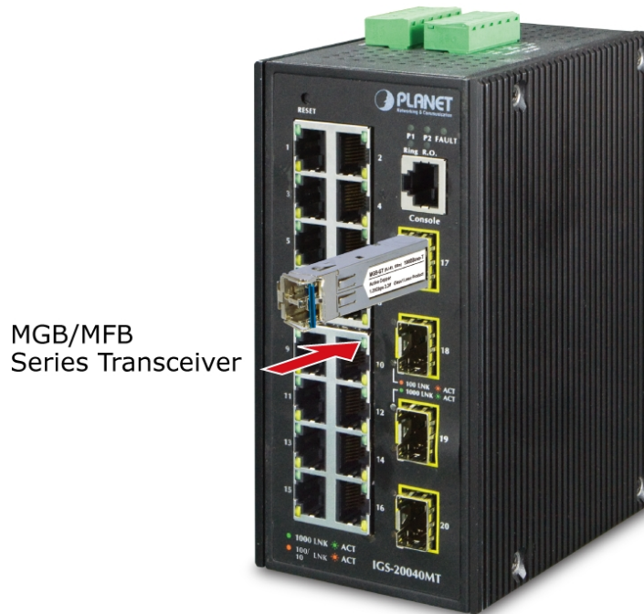
Figure 2-18: Plugging in the SFP/SFP+ Transceiver
