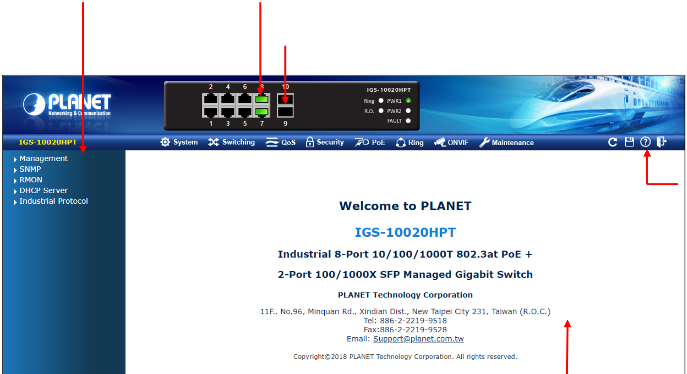
Figure 4-1-4: Main page
