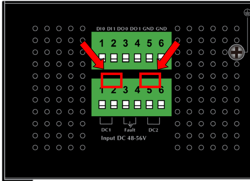
Figure 2-13: IGS-20160HPT Upper Panel
