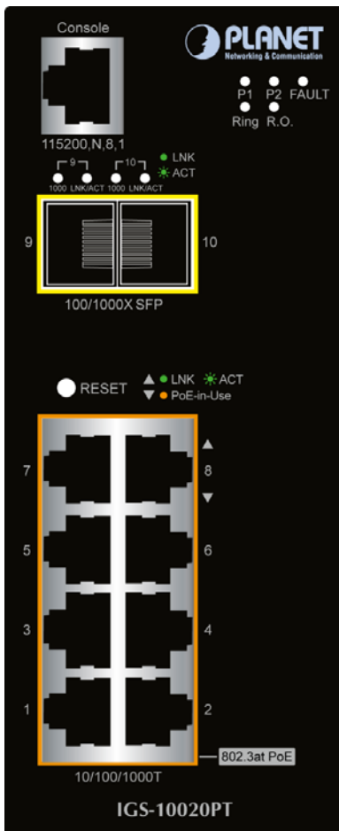
Figure 2-1: IGS-10020PT Switch Front Panel
