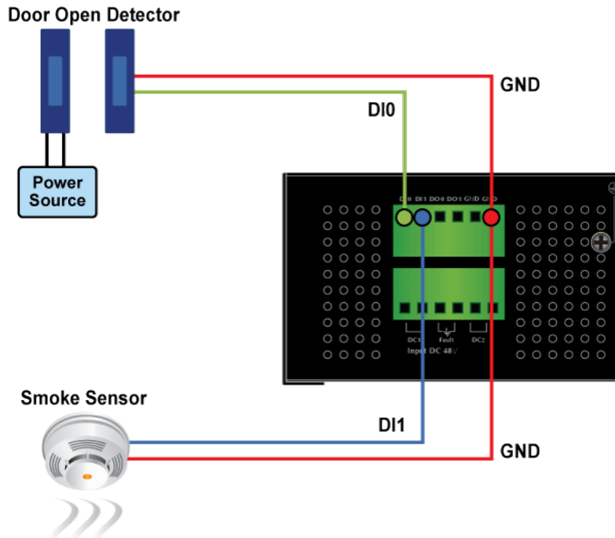
Figure 2-16: Wiring DI0 and DI1 to Open Detector
