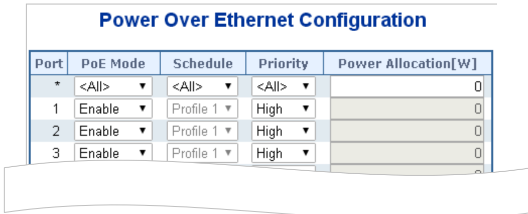
Figure 4-6-1-3: Power over Ethernet Configuration Screenshot
