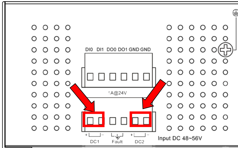
Figure 2-11: IGS-10020PT Upper Panel
