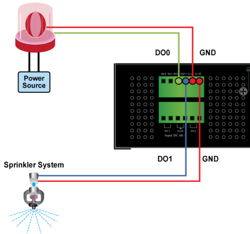
Figure 2-17: Wiring DO0 and DO1 to Open Detector
