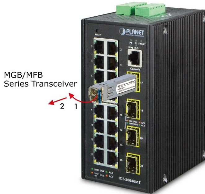
Figure 2-19: Pulling out the SFP/SFP+ Transceiver Module
