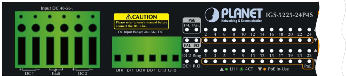
Figure 2-11: IGS-5225-24P4S LED on Front Panel
