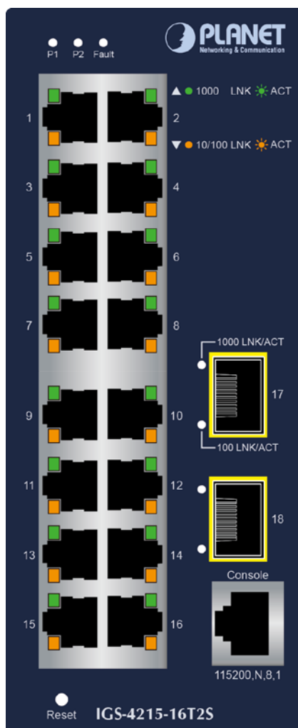
Figure 2-1-3: LED Panel
