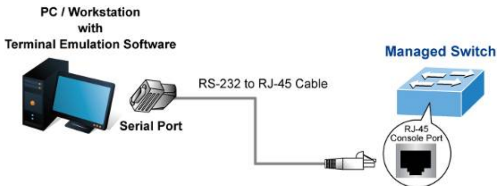
Figure 3-1-1: Console Management
