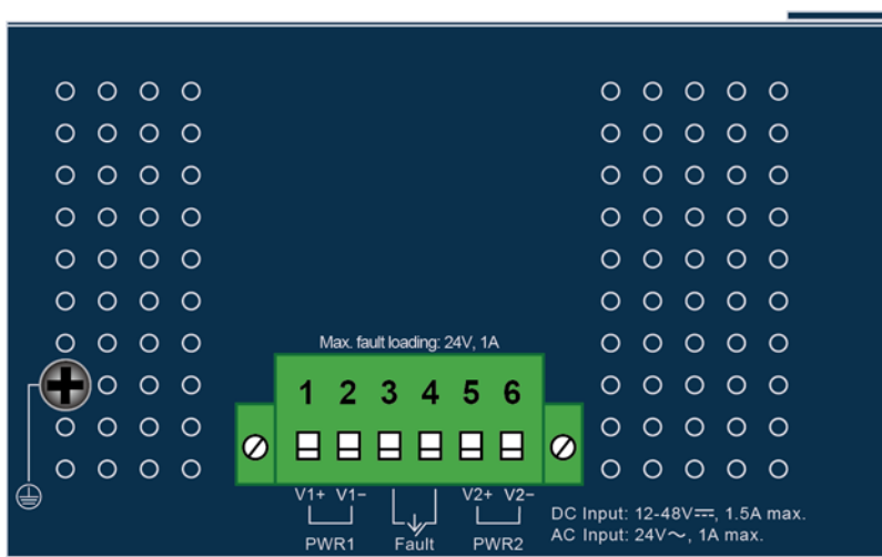
Figure 2-1-4: Top View
