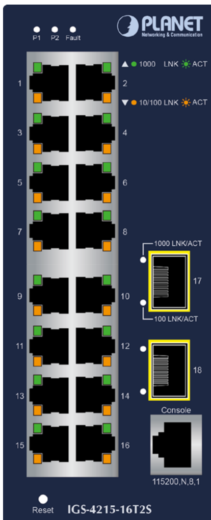
Figure 2-1-2: Front Panel
