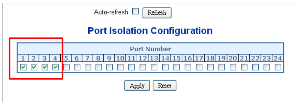
Figure 4-6-17: The Configuration of Isolated and Promiscuous Port
