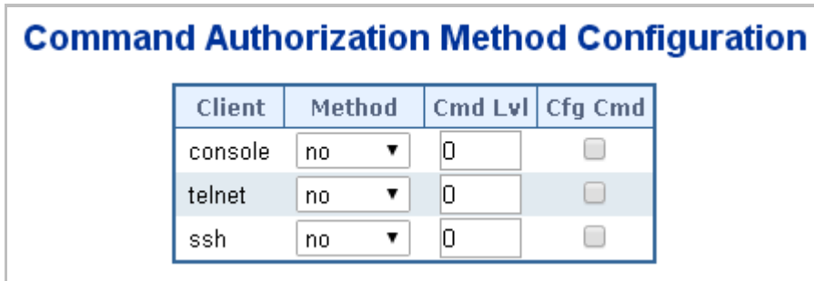
Figure 4-11-4 : Command Authorization Method Configuration page Screenshot
