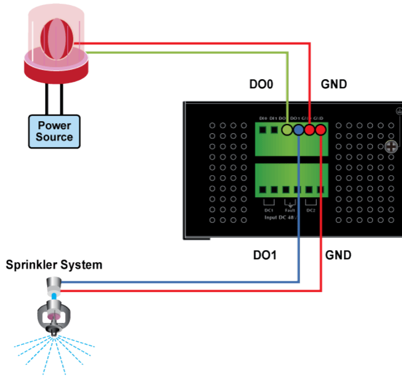
Figure 2-17 Wires DO0 and DO1 to Open Detector
