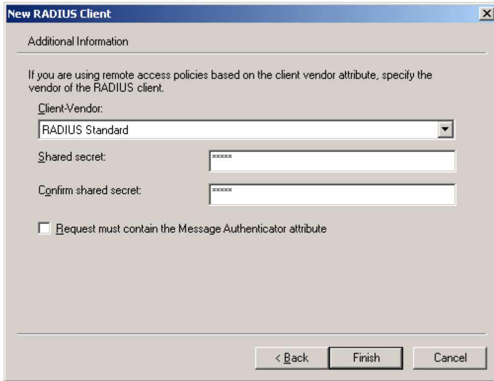
Figure 4-11-17: Windows Server RADIUS Server Setting
